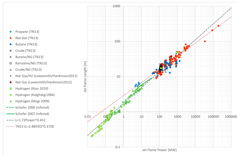
Figure 4: Flame length plotted against jet fire power
