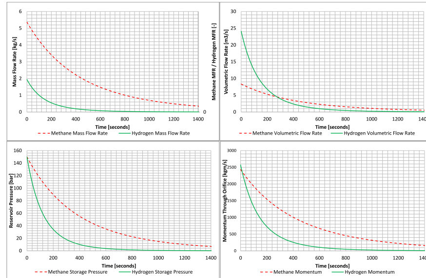
Figure 1: Vessel and release properties for hydrogen and methane (mass release rate – top left, volumetric flow – top right, vessel pressure – bottom left and release momentum – bottom right)
