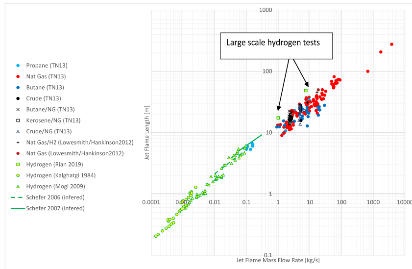
Figure 3: Flame length plotted against mass release rate
