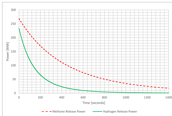
Figure 2: Release power variation with time
