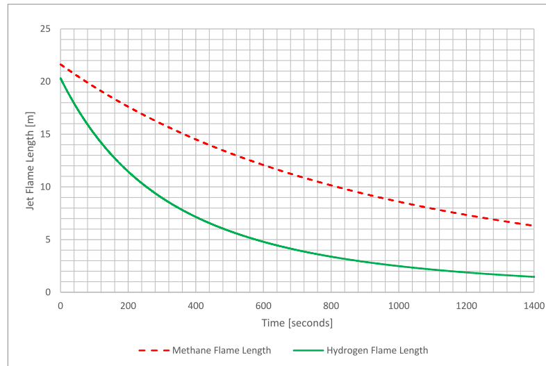
Figure 5: Flame lengths
